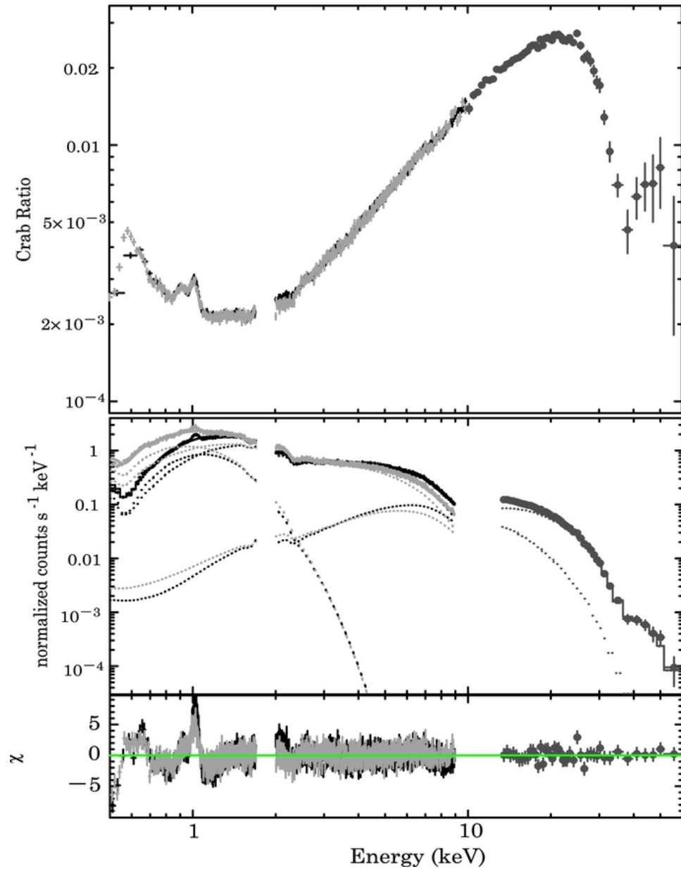
Figure 2. from Possible Detection of an Emission Cyclotron Resonance Scattering Feature from the Accretion-powered Pulsar 4U 1626–67 Iwakiri et al. 2012 ApJ 751 35 doi:10.1088/0004-637X/751/1/35 https://dx.doi.org/10.1088/0004-637X/751/1/35 © 2012. The American Astronomical Society. All rights reserved.
