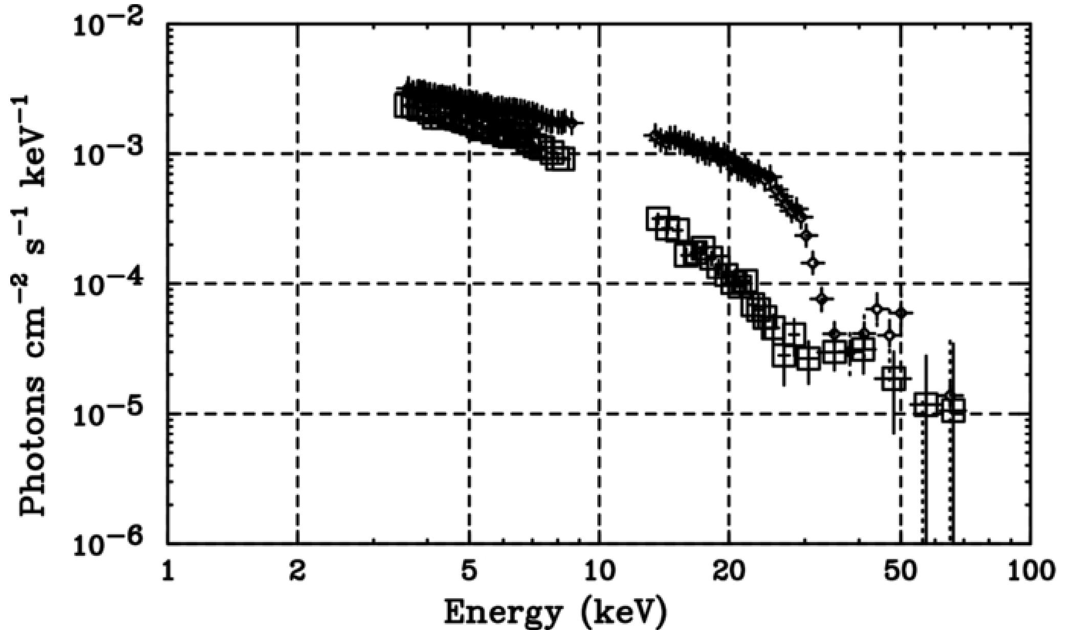
Figure 13. from Possible Detection of an Emission Cyclotron Resonance Scattering Feature from the Accretion-powered Pulsar 4U 1626–67 Iwakiri et al. 2012 ApJ 751 35 doi:10.1088/0004-637X/751/1/35 https://dx.doi.org/10.1088/0004-637X/751/1/35 © 2012. The American Astronomical Society. All rights reserved.
