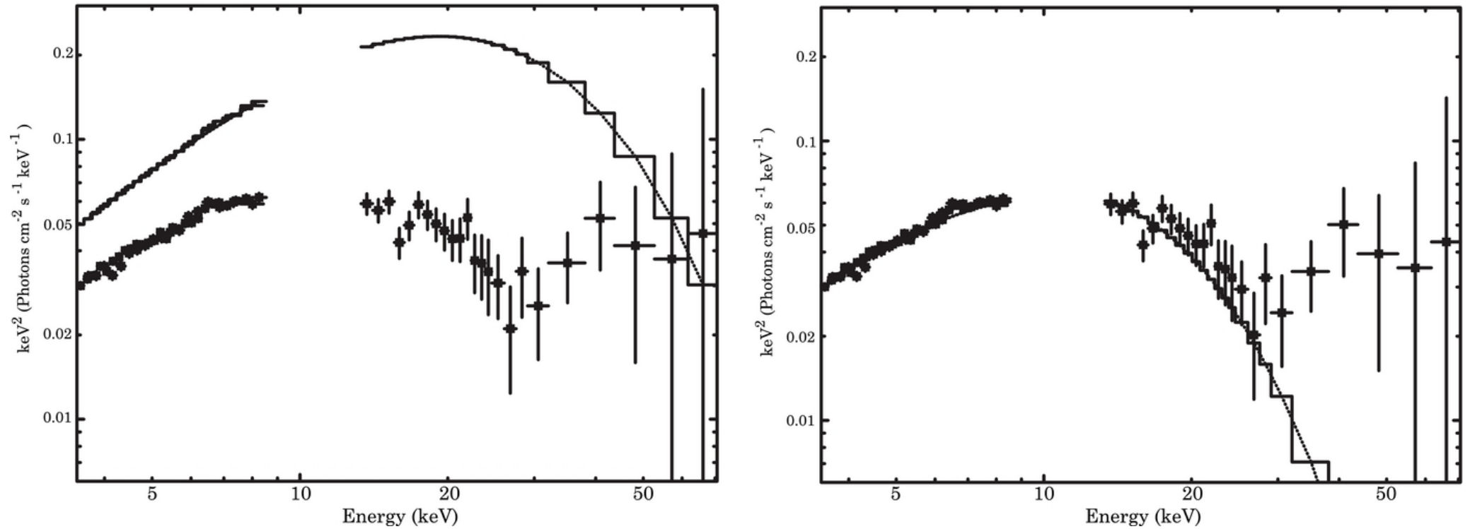
Figure 12. from Possible Detection of an Emission Cyclotron Resonance Scattering Feature from the Accretion-powered Pulsar 4U 1626–67 Iwakiri et al. 2012 ApJ 751 35 doi:10.1088/0004-637X/751/1/35 https://dx.doi.org/10.1088/0004-637X/751/1/35 © 2012. The American Astronomical Society. All rights reserved.
