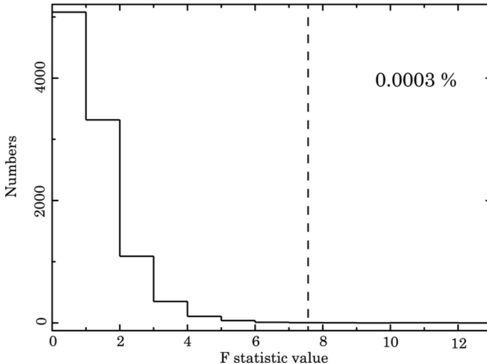
Figure 11. from Possible Detection of an Emission Cyclotron Resonance Scattering Feature from the Accretion-powered Pulsar 4U 1626–67 Iwakiri et al. 2012 ApJ 751 35 doi:10.1088/0004-637X/751/1/35 https://dx.doi.org/10.1088/0004-637X/751/1/35 © 2012. The American Astronomical Society. All rights reserved.
