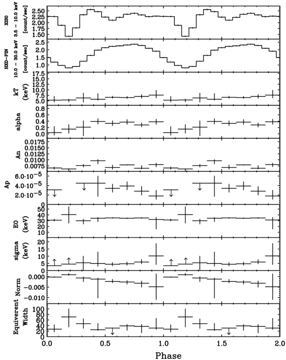
Figure 10. from Possible Detection of an Emission Cyclotron Resonance Scattering Feature from the Accretion-powered Pulsar 4U 1626–67 Iwakiri et al. 2012 ApJ 751 35 doi:10.1088/0004-637X/751/1/35 https://dx.doi.org/10.1088/0004-637X/751/1/35 © 2012. The American Astronomical Society. All rights reserved.
