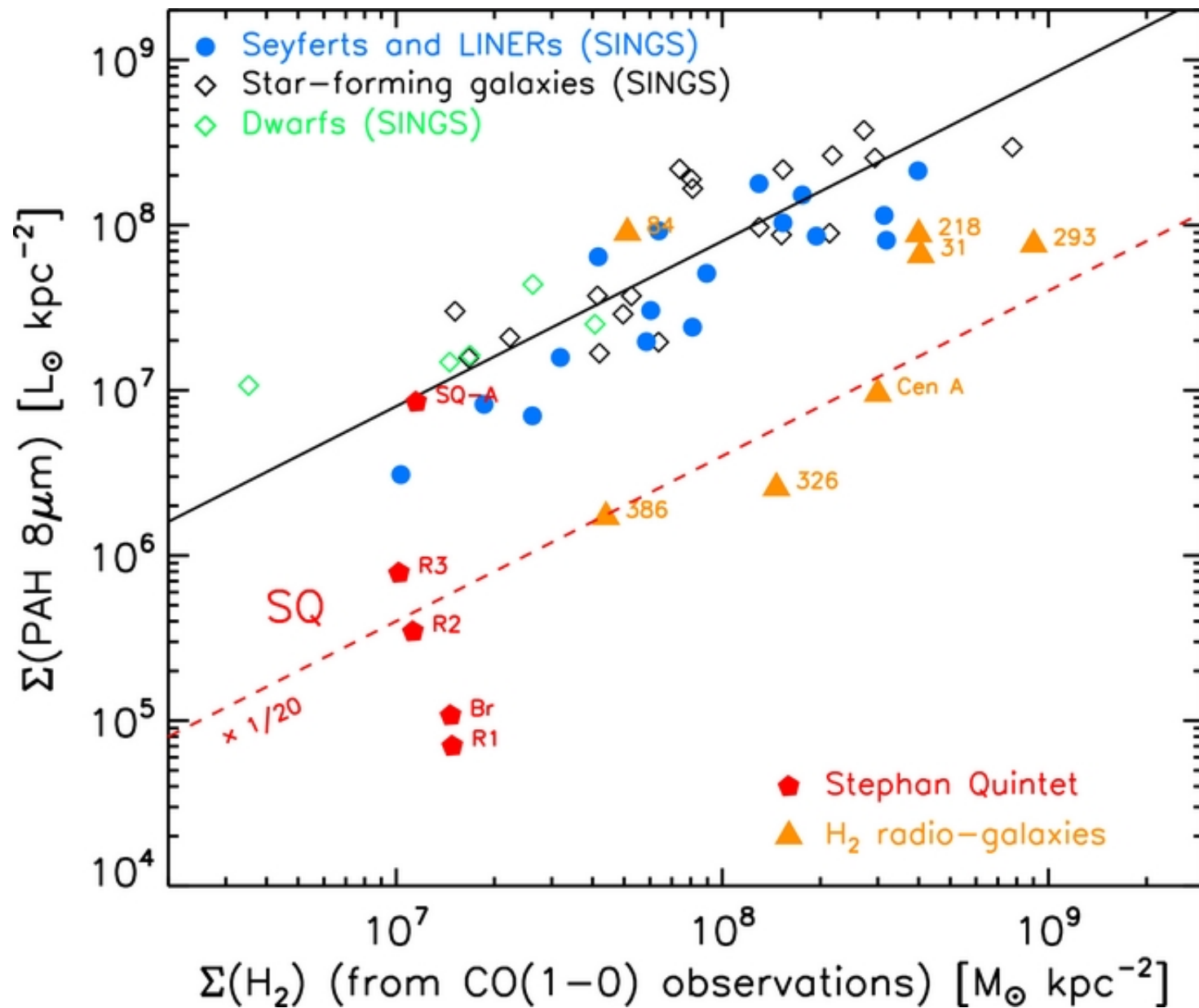
Figure 5. from Turbulent Molecular Gas and Star Formation in the Shocked Intergalactic Medium of Stephan's Quintet Guillard et al. 2012 ApJ 749 158 doi:10.1088/0004-637X/749/2/158 https://dx.doi.org/10.1088/0004-637X/749/2/158 © 2012. The American Astronomical Society. All rights reserved.
