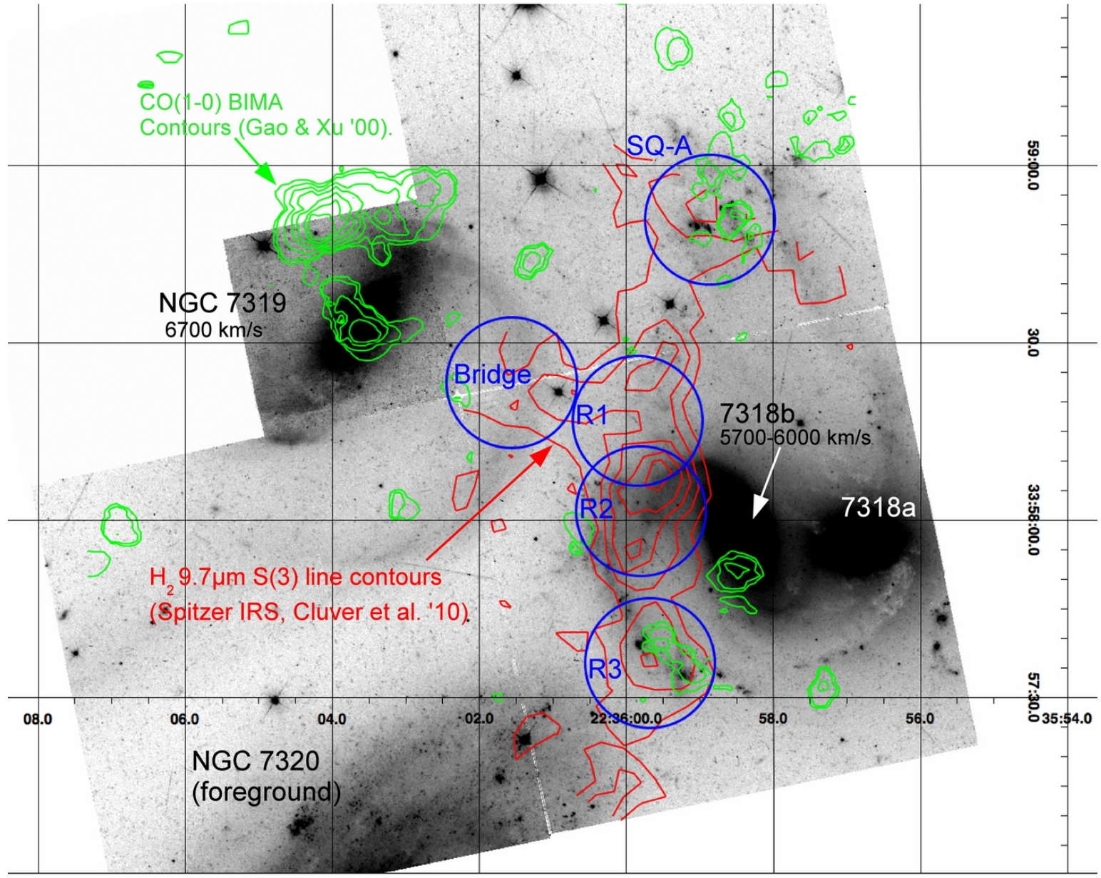
Figure 1. from Turbulent Molecular Gas and Star Formation in the Shocked Intergalactic Medium of Stephan's Quintet Guillard et al. 2012 ApJ 749 158 doi:10.1088/0004-637X/749/2/158 https://dx.doi.org/10.1088/0004-637X/749/2/158 © 2012. The American Astronomical Society. All rights reserved.
