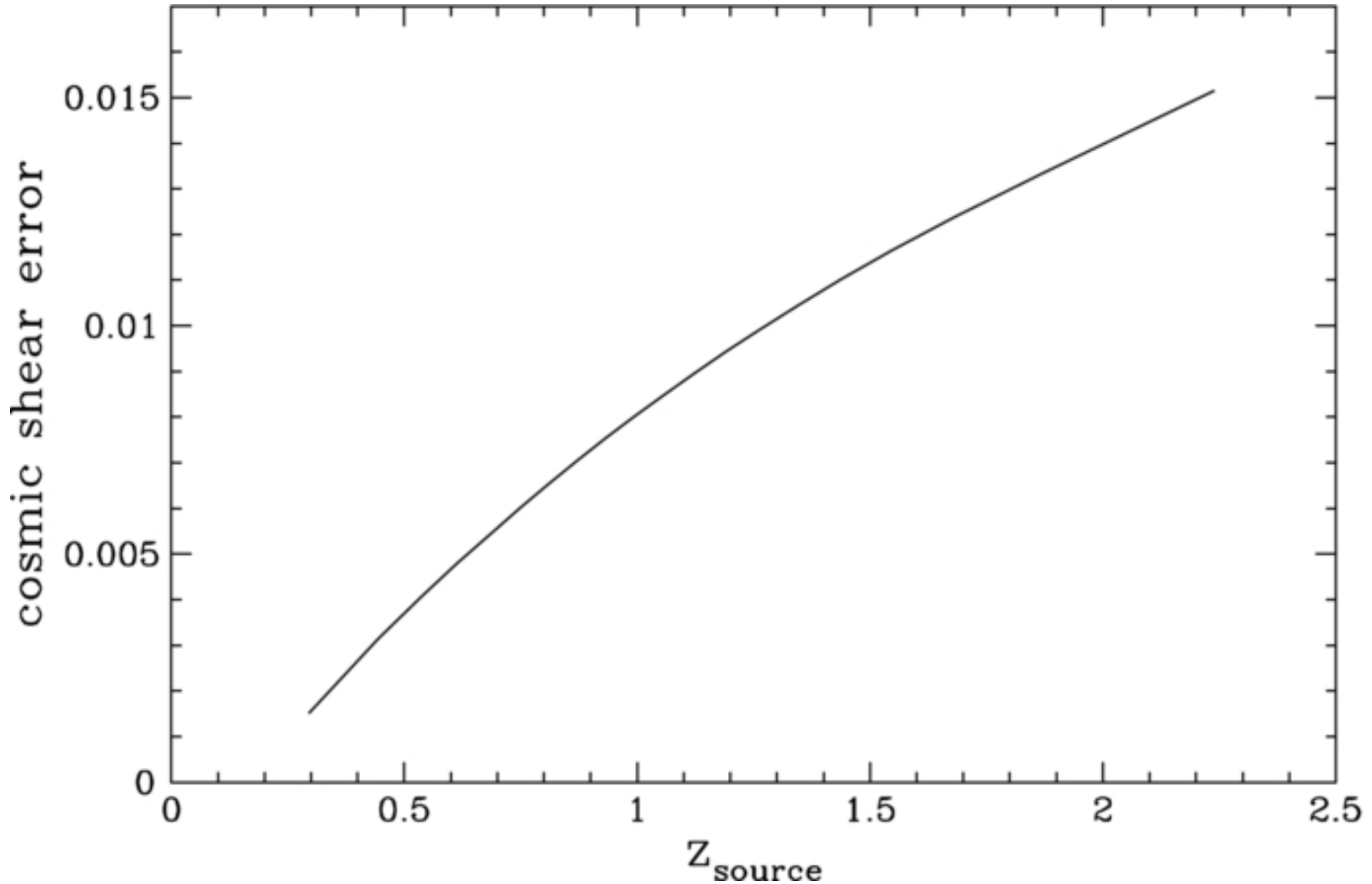
Figure 7. from Measuring the Geometry of the Universe from Weak Gravitational Lensing behind Galaxy Groups in the HST COSMOS Survey Taylor et al. 2012 ApJ 749 127 doi:10.1088/0004-637X/749/2/127 https://dx.doi.org/10.1088/0004-637X/749/2/127 © 2012. The American Astronomical Society. All rights reserved.
