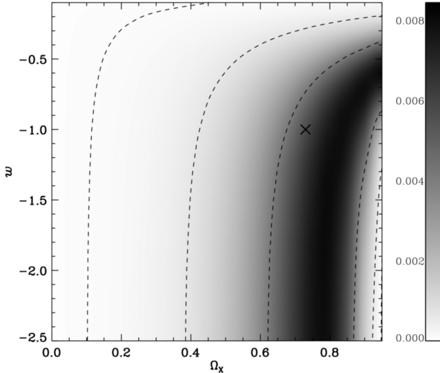
Figure 6. from Measuring the Geometry of the Universe from Weak Gravitational Lensing behind Galaxy Groups in the HST COSMOS Survey Taylor et al. 2012 ApJ 749 127 doi:10.1088/0004-637X/749/2/127 https://dx.doi.org/10.1088/0004-637X/749/2/127 © 2012. The American Astronomical Society. All rights reserved.
