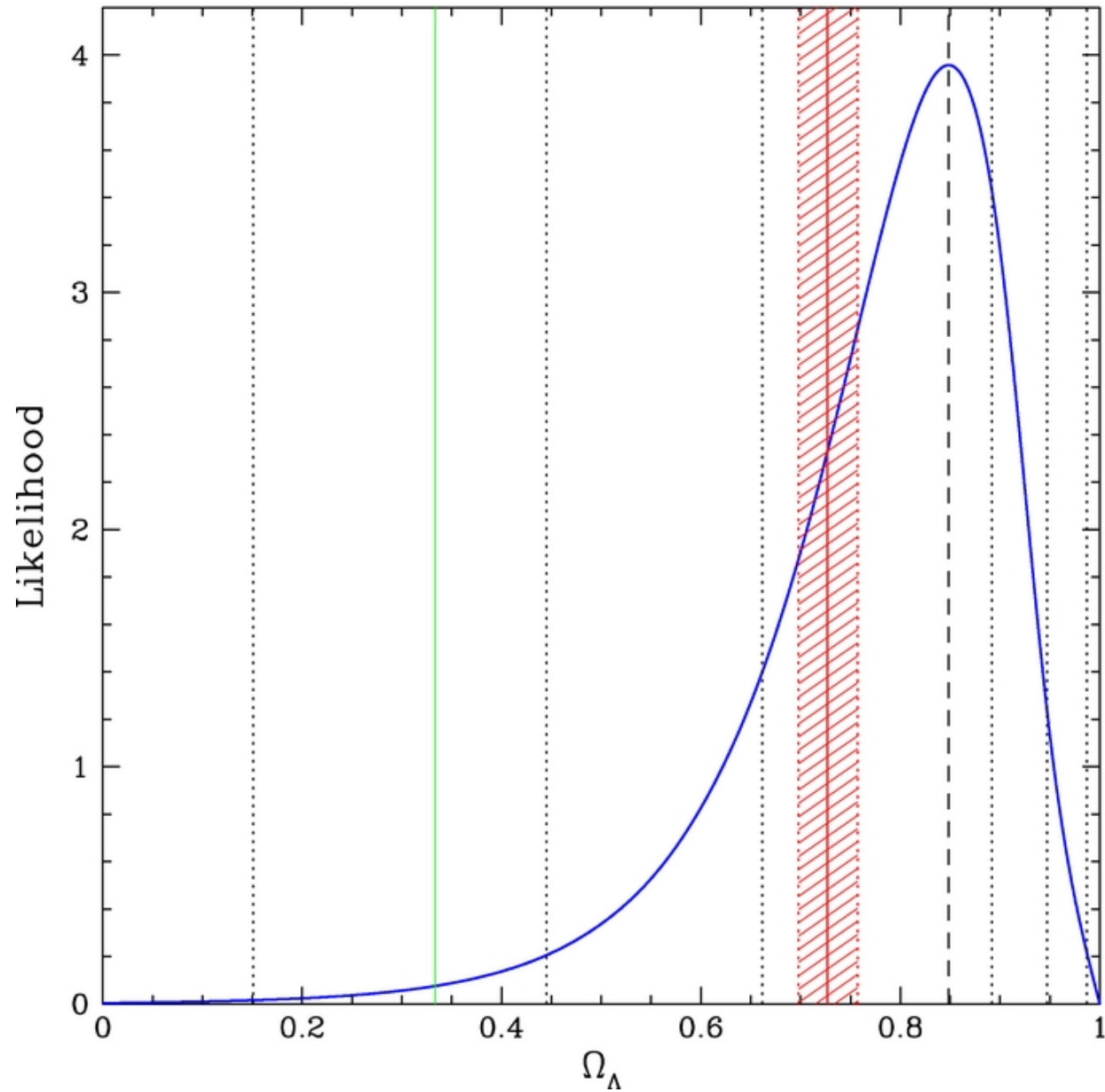
Figure 5. from Measuring the Geometry of the Universe from Weak Gravitational Lensing behind Galaxy Groups in the HST COSMOS Survey Taylor et al. 2012 ApJ 749 127 doi:10.1088/0004-637X/749/2/127 https://dx.doi.org/10.1088/0004-637X/749/2/127 © 2012. The American Astronomical Society. All rights reserved.
