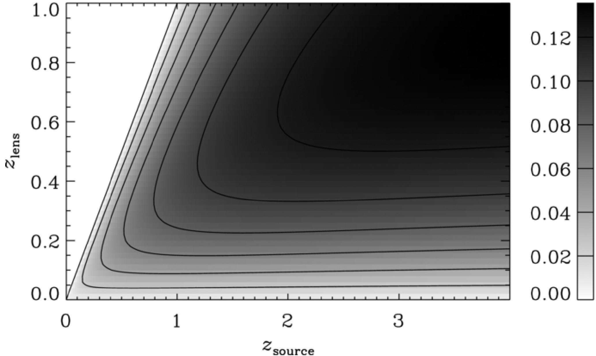
Figure 4. from Measuring the Geometry of the Universe from Weak Gravitational Lensing behind Galaxy Groups in the HST COSMOS Survey Taylor et al. 2012 ApJ 749 127 doi:10.1088/0004-637X/749/2/127 https://dx.doi.org/10.1088/0004-637X/749/2/127 © 2012. The American Astronomical Society. All rights reserved.
