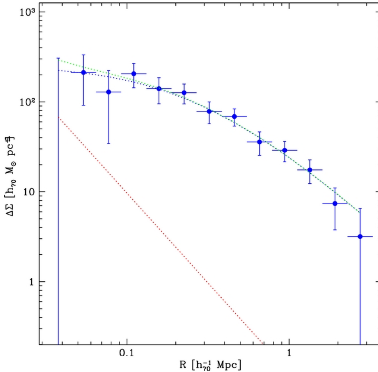
Figure 2. from Measuring the Geometry of the Universe from Weak Gravitational Lensing behind Galaxy Groups in the HST COSMOS Survey Taylor et al. 2012 ApJ 749 127 doi:10.1088/0004-637X/749/2/127 https://dx.doi.org/10.1088/0004-637X/749/2/127 © 2012. The American Astronomical Society. All rights reserved.
