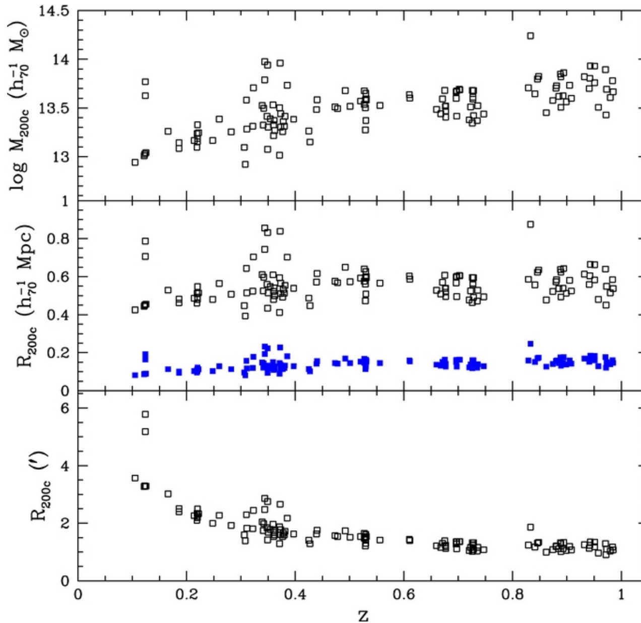
Figure 1. from Measuring the Geometry of the Universe from Weak Gravitational Lensing behind Galaxy Groups in the HST COSMOS Survey Taylor et al. 2012 ApJ 749 127 doi:10.1088/0004-637X/749/2/127 https://dx.doi.org/10.1088/0004-637X/749/2/127 © 2012. The American Astronomical Society. All rights reserved.
