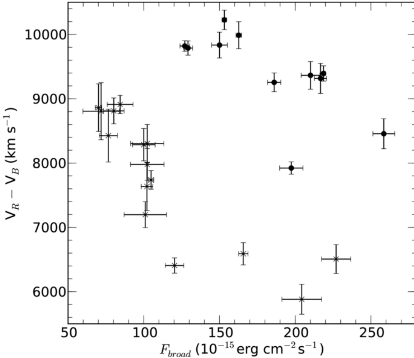
Figure 7. from Short Timescale Variations of the H Double-peaked Profile of the Nucleus of NGC 1097 Schimoia et al. 2012 ApJ 748 145 doi:10.1088/0004-637X/748/2/145 https://dx.doi.org/10.1088/0004-637X/748/2/145 © 2012. The American Astronomical Society. All rights reserved.
