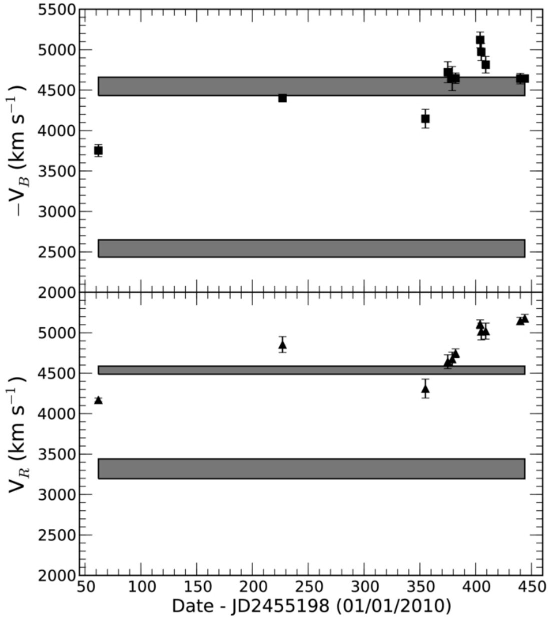
Figure 4. from Short Timescale Variations of the H Double-peaked Profile of the Nucleus of NGC 1097 Schimoia et al. 2012 ApJ 748 145 doi:10.1088/0004-637X/748/2/145 https://dx.doi.org/10.1088/0004-637X/748/2/145 © 2012. The American Astronomical Society. All rights reserved.
