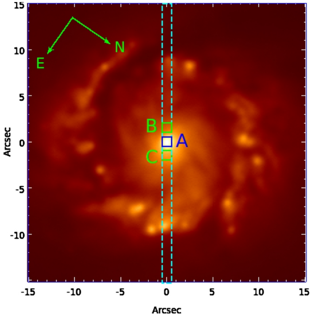
Figure 1. from Short Timescale Variations of the H Double-peaked Profile of the Nucleus of NGC 1097 Schimoia et al. 2012 ApJ 748 145 doi:10.1088/0004-637X/748/2/145 https://dx.doi.org/10.1088/0004-637X/748/2/145 © 2012. The American Astronomical Society. All rights reserved.
