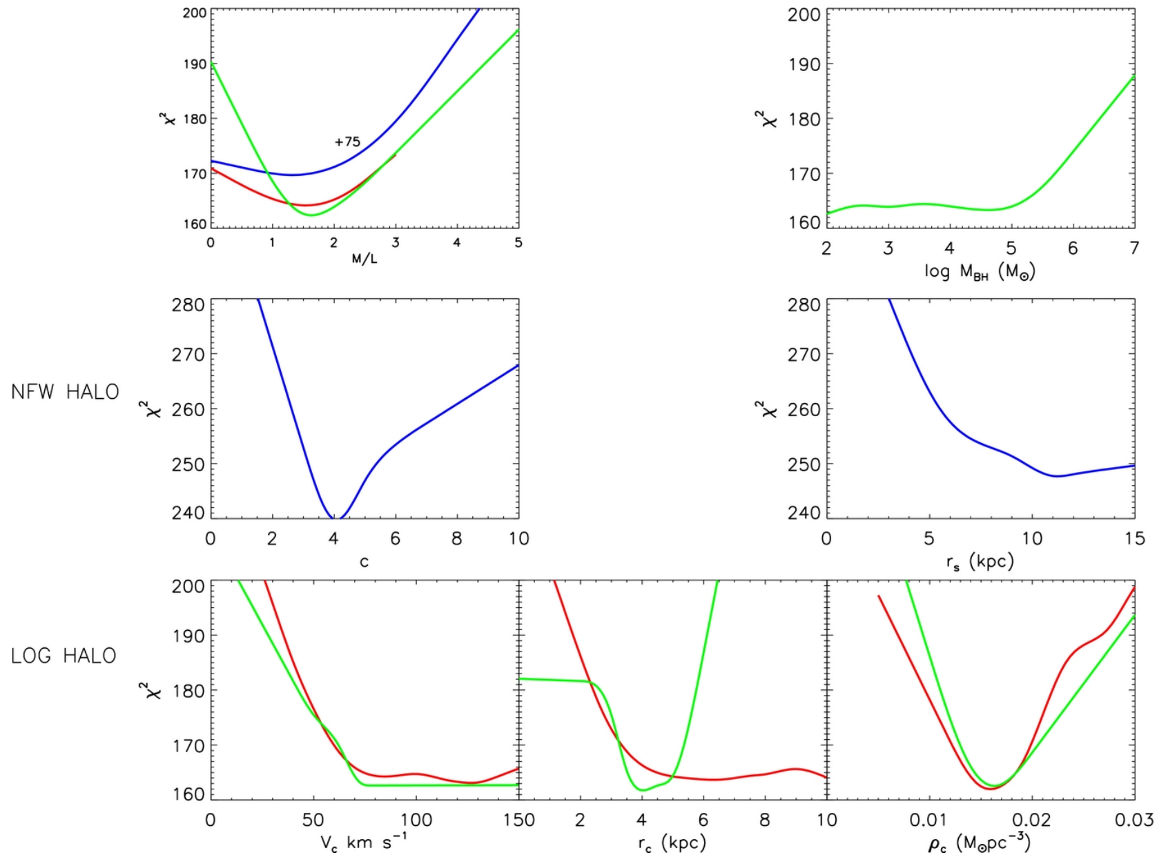
Figure 3. from The Dark Matter Density Profile of the Fornax Dwarf Jardel & Gebhardt 2012 ApJ 746 89 doi:10.1088/0004-637X/746/1/89 https://dx.doi.org/10.1088/0004-637X/746/1/89 © 2012. The American Astronomical Society. All rights reserved.
