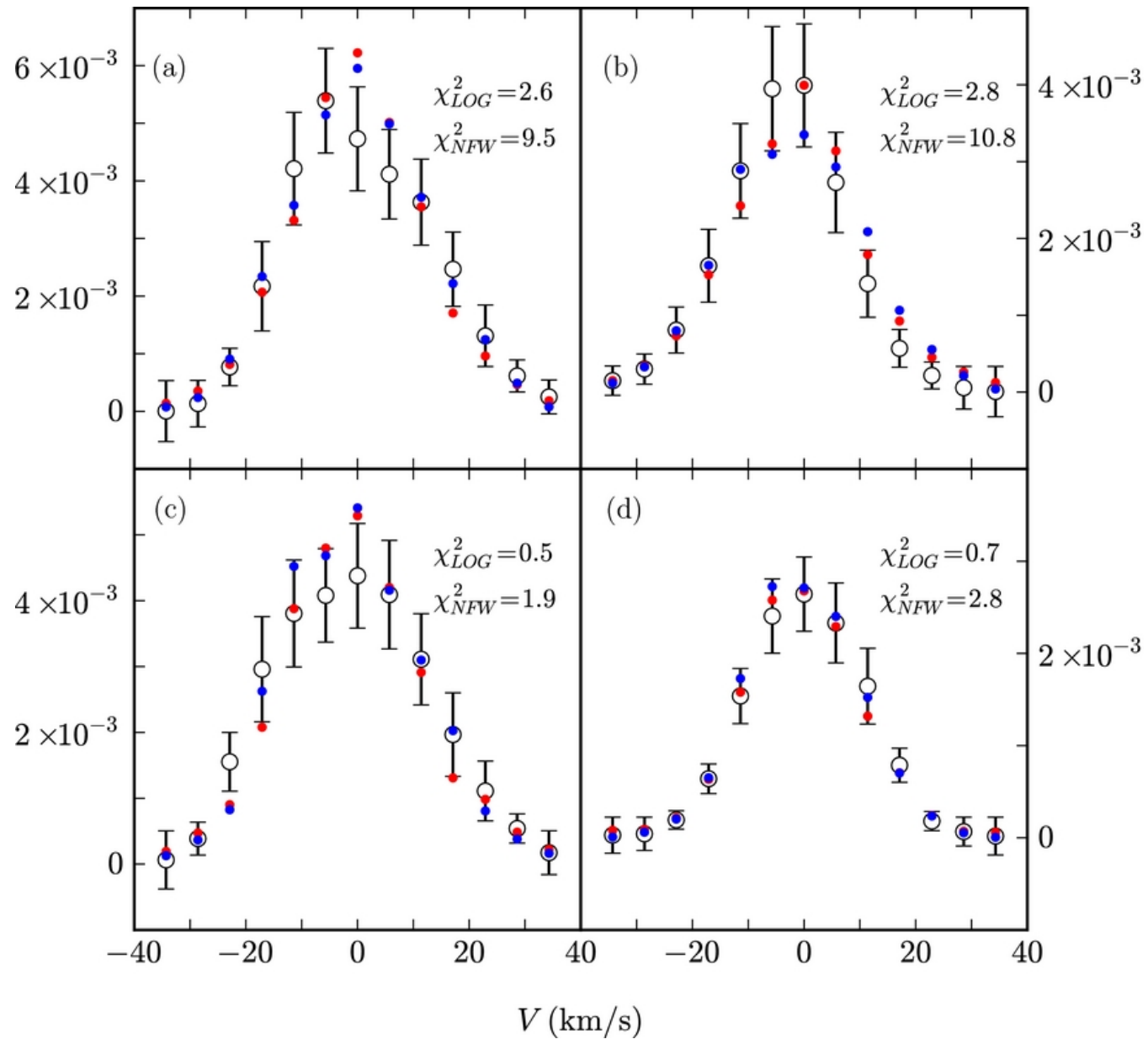
Figure 1. from The Dark Matter Density Profile of the Fornax Dwarf Jardel & Gebhardt 2012 ApJ 746 89 doi:10.1088/0004-637X/746/1/89 https://dx.doi.org/10.1088/0004-637X/746/1/89 © 2012. The American Astronomical Society. All rights reserved.
