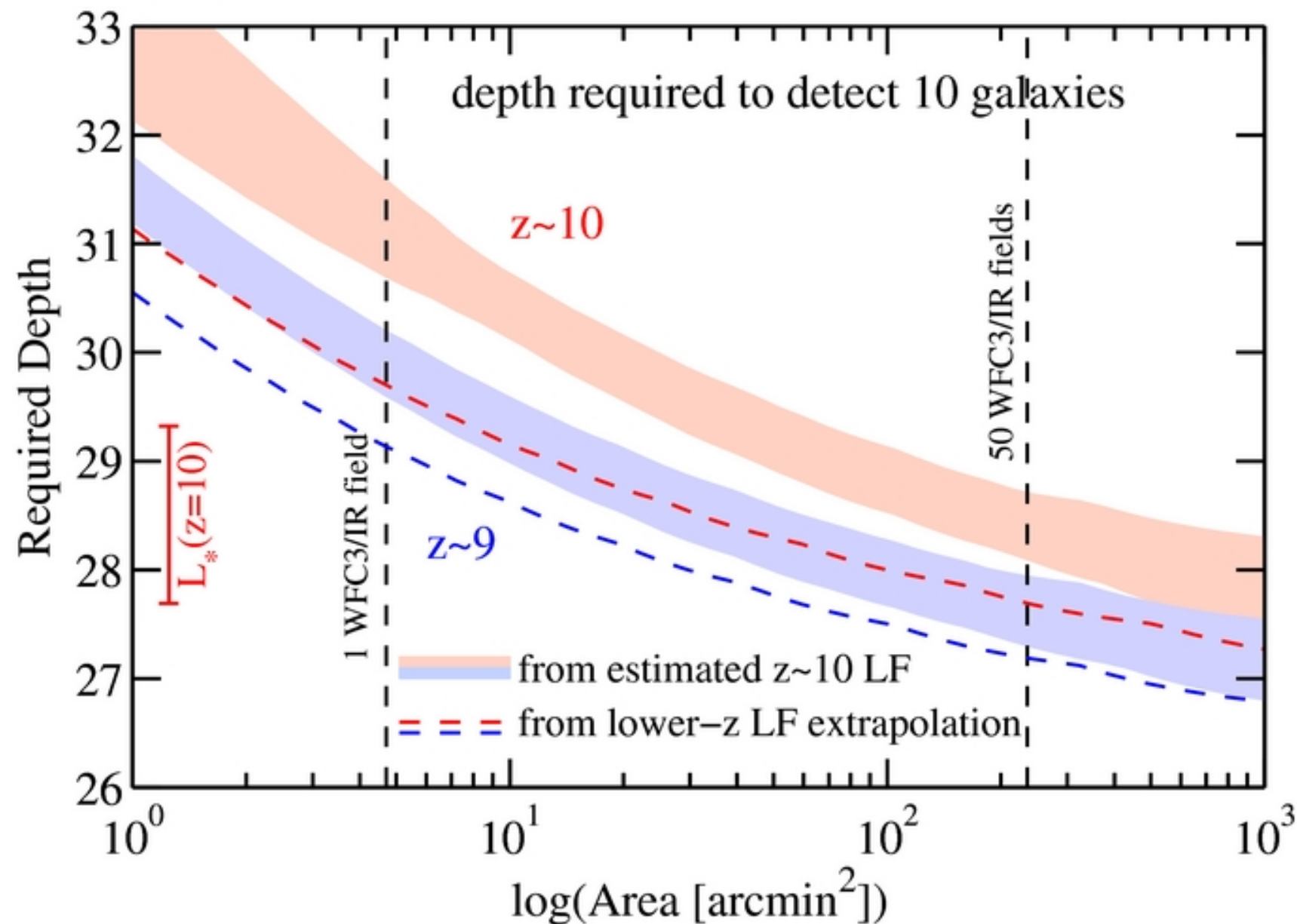
Figure 9. from Expanded Search for z \sim 10 Galaxies from HUDF09, ERS, and CANDELS Data: Evidence for Accelerated Evolution at z > 8 ? Oesch et al. 2012 ApJ 745 110 doi:10.1088/0004-637X/745/2/110 https://dx.doi.org/10.1088/0004-637X/745/2/110 © 2012. The American Astronomical Society. All rights reserved.
