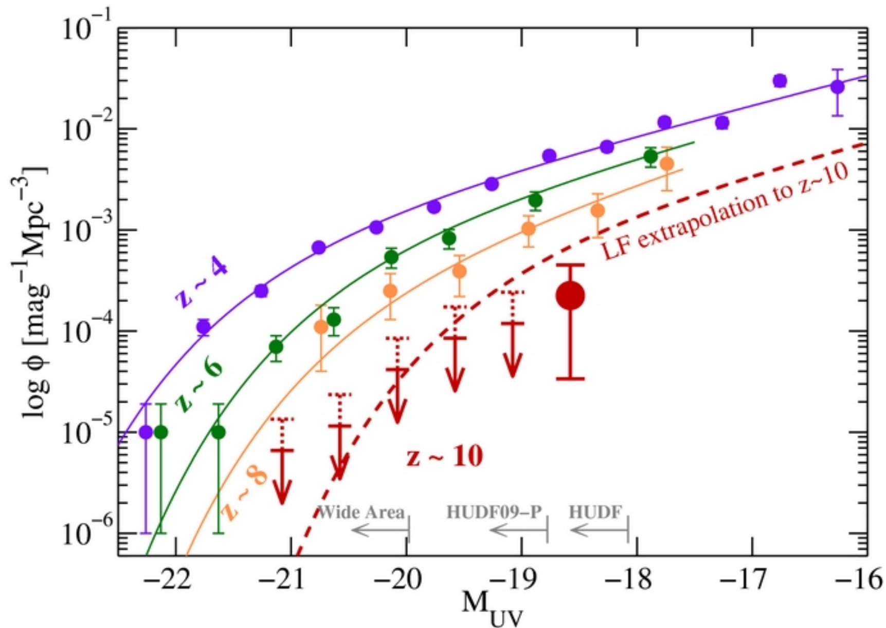
Figure 7. from Expanded Search for z \gtrsim 10 Galaxies from HUDF09, ERS, and CANDELS Data: Evidence for Accelerated Evolution at z > 8 ? Oesch et al. 2012 ApJ 745 110 doi:10.1088/0004-637X/745/2/110 https://dx.doi.org/10.1088/0004-637X/745/2/110 © 2012. The American Astronomical Society. All rights reserved.
