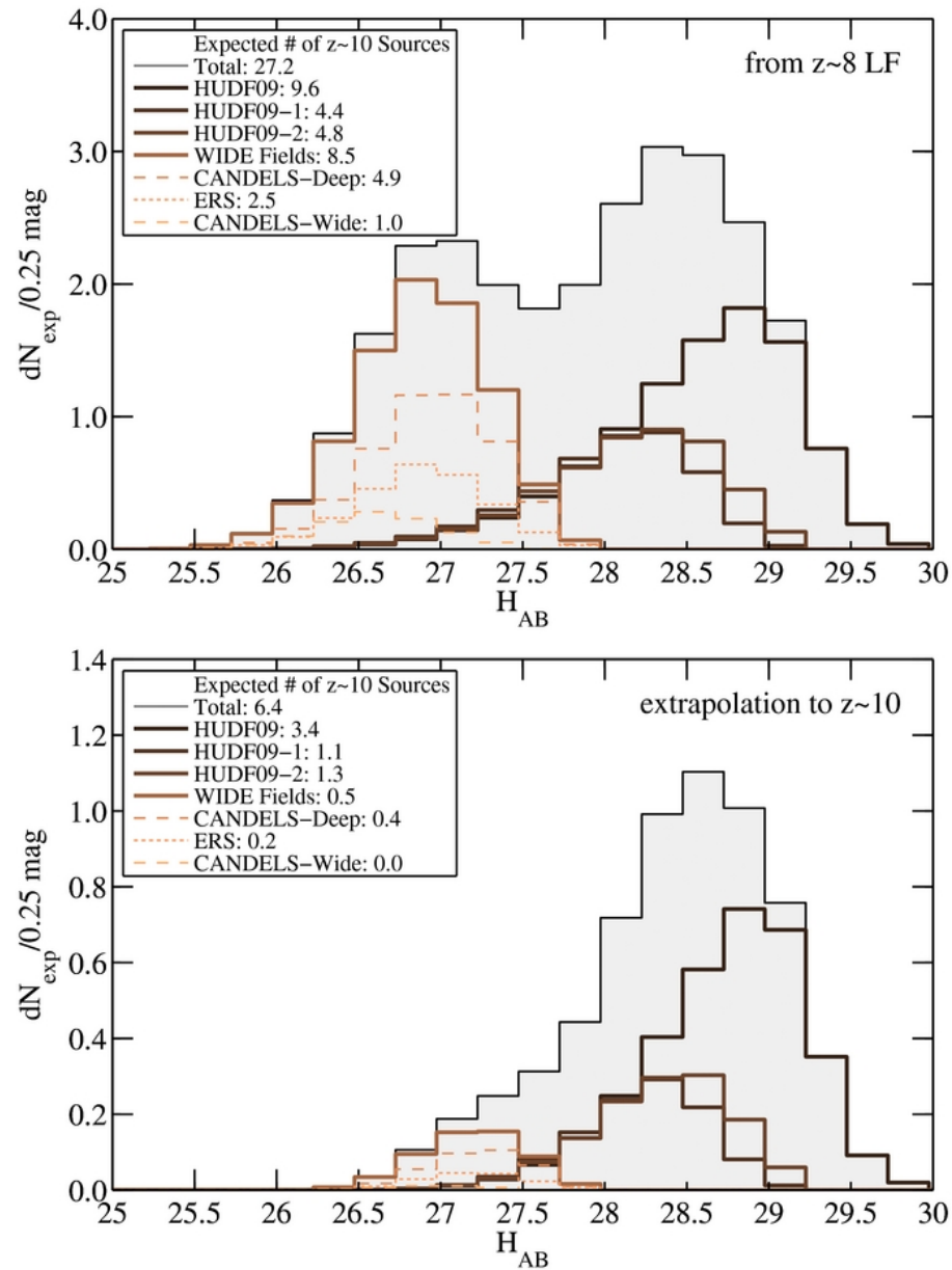
Figure 6. from Expanded Search for z \sim 10 Galaxies from HUDF09, ERS, and CANDELS Data: Evidence for Accelerated Evolution at z > 8 ? Oesch et al. 2012 ApJ 745 110 doi:10.1088/0004-637X/745/2/110 https://dx.doi.org/10.1088/0004-637X/745/2/110 © 2012. The American Astronomical Society. All rights reserved.
