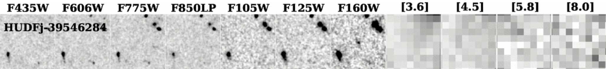
Figure 4. from Expanded Search for z \sim 10 Galaxies from HUDF09, ERS, and CANDELS Data: Evidence for Accelerated Evolution at z > 8 ? Oesch et al. 2012 ApJ 745 110 doi:10.1088/0004-637X/745/2/110 https://dx.doi.org/10.1088/0004-637X/745/2/110 © 2012. The American Astronomical Society. All rights reserved.
