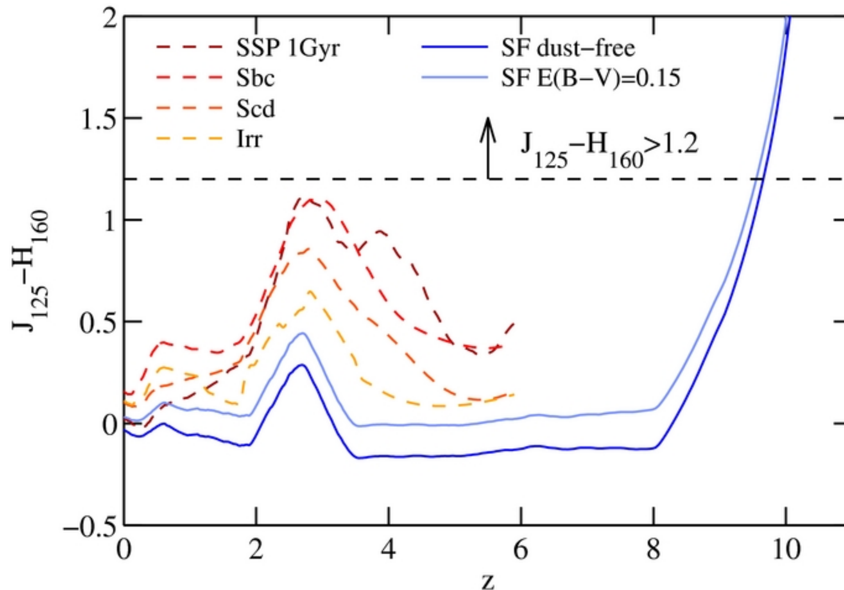
Figure 2. from Expanded Search for z > 10 Galaxies from HUDF09, ERS, and CANDELS Data: Evidence for Accelerated Evolution at z > 8 ? Oesch et al. 2012 ApJ 745 110 doi:10.1088/0004-637X/745/2/110 https://dx.doi.org/10.1088/0004-637X/745/2/110 © 2012. The American Astronomical Society. All rights reserved.
