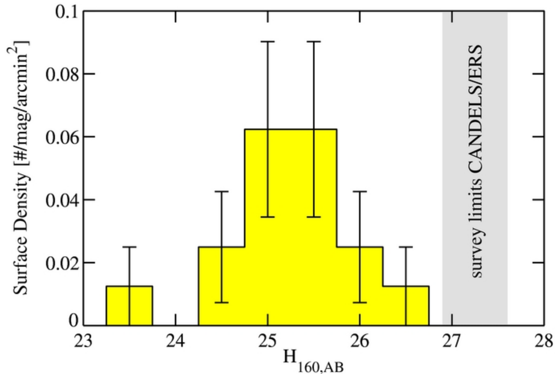
Figure 11. from Expanded Search for z \gtrsim 10 Galaxies from HUDF09, ERS, and CANDELS Data: Evidence for Accelerated Evolution at z > 8 ? Oesch et al. 2012 ApJ 745 110 doi:10.1088/0004-637X/745/2/110 https://dx.doi.org/10.1088/0004-637X/745/2/110 © 2012. The American Astronomical Society. All rights reserved.
