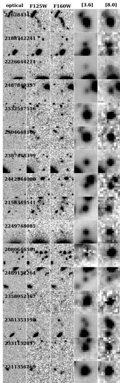
Figure 10. from Expanded Search for z \sim 10 Galaxies from HUDF09, ERS, and CANDELS Data: Evidence for Accelerated Evolution at z > 8 ? Oesch et al. 2012 ApJ 745 110 doi:10.1088/0004-637X/745/2/110 https://dx.doi.org/10.1088/0004-637X/745/2/110 © 2012. The American Astronomical Society. All rights reserved.
