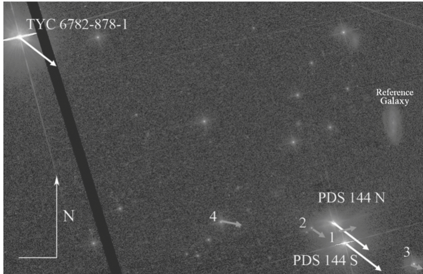
Figure 5. from PDS 144: The First Confirmed Herbig Ae-Herbig Ae Wide Binary Hornbeck et al. 2012 ApJ 744 54 doi:10.1088/0004-637X/744/1/54 https://dx.doi.org/10.1088/0004-637X/744/1/54 © 2012. The American Astronomical Society. All rights reserved.
