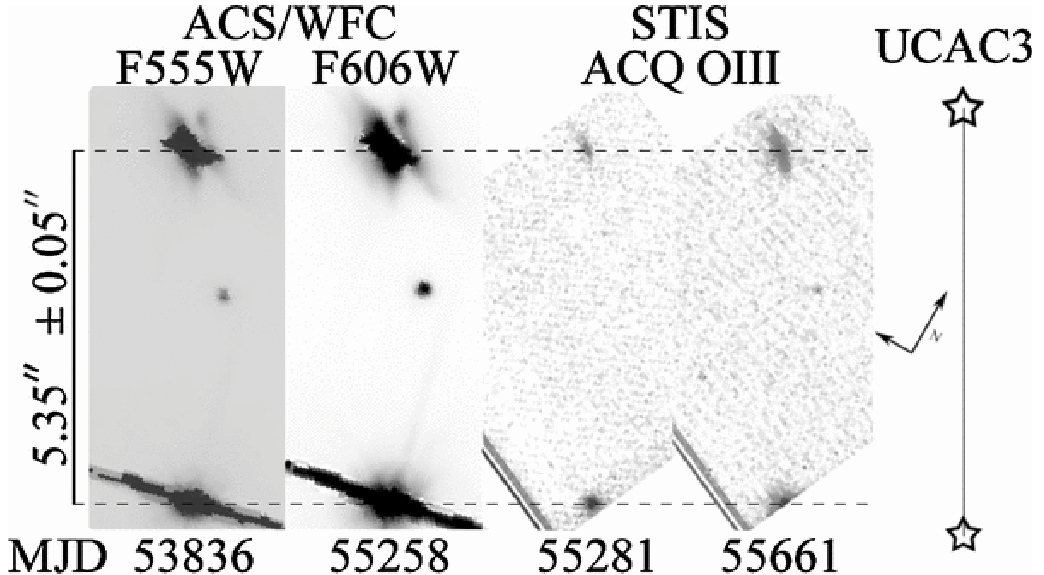
Figure 3. from PDS 144: The First Confirmed Herbig Ae-Herbig Ae Wide Binary Hornbeck et al. 2012 ApJ 744 54 doi:10.1088/0004-637X/744/1/54 https://dx.doi.org/10.1088/0004-637X/744/1/54 © 2012. The American Astronomical Society. All rights reserved.
