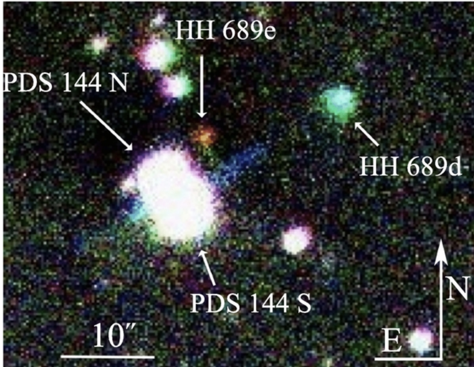
Figure 2. from PDS 144: The First Confirmed Herbig Ae-Herbig Ae Wide Binary Hornbeck et al. 2012 ApJ 744 54 doi:10.1088/0004-637X/744/1/54 https://dx.doi.org/10.1088/0004-637X/744/1/54 © 2012. The American Astronomical Society. All rights reserved.
