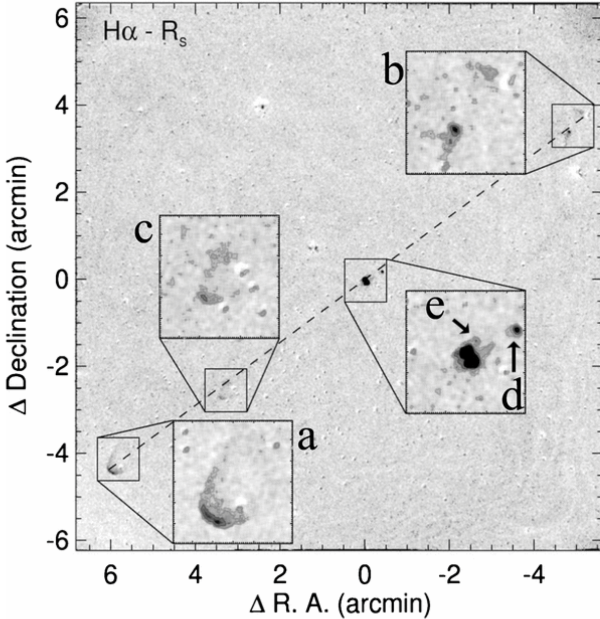
Figure 1. from PDS 144: The First Confirmed Herbig Ae-Herbig Ae Wide Binary Hornbeck et al. 2012 ApJ 744 54 doi:10.1088/0004-637X/744/1/54 https://dx.doi.org/10.1088/0004-637X/744/1/54 © 2012. The American Astronomical Society. All rights reserved.
