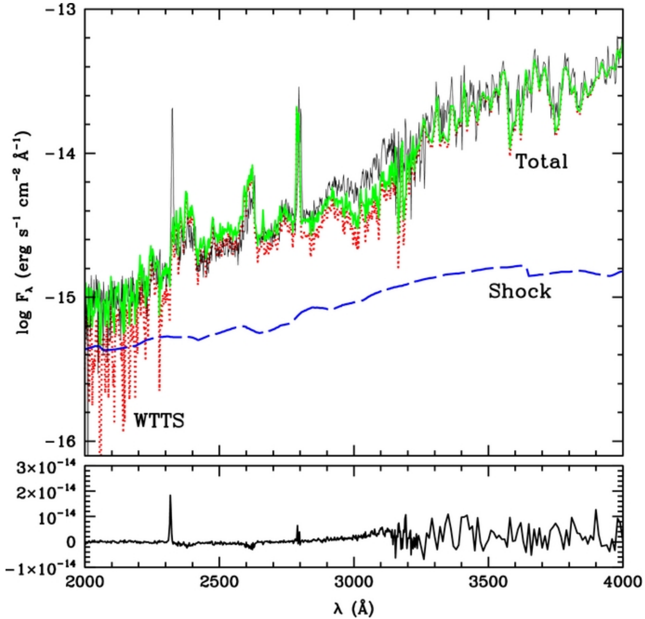
Figure 8. from Near-ultraviolet Excess in Slowly Accreting T Tauri Stars: Limits Imposed by Chromospheric Emission Ingleby et al. 2011 ApJ 743 105 doi:10.1088/0004-637X/743/2/105 https://dx.doi.org/10.1088/0004-637X/743/2/105 © 2011. The American Astronomical Society. All rights reserved.
