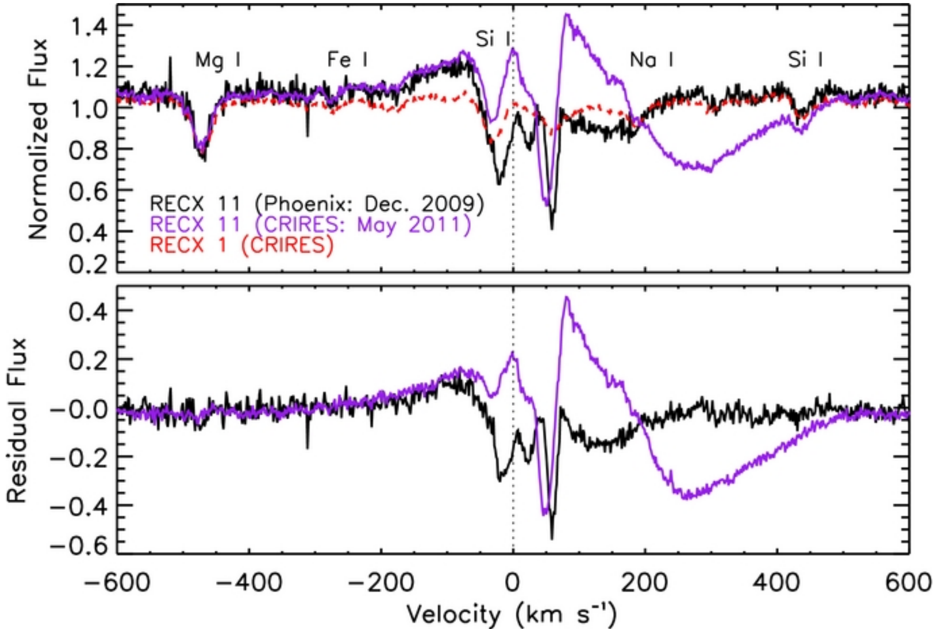
Figure 3. from Near-ultraviolet Excess in Slowly Accreting T Tauri Stars: Limits Imposed by Chromospheric Emission Ingleby et al. 2011 ApJ 743 105 doi:10.1088/0004-637X/743/2/105 https://dx.doi.org/10.1088/0004-637X/743/2/105 © 2011. The American Astronomical Society. All rights reserved.
