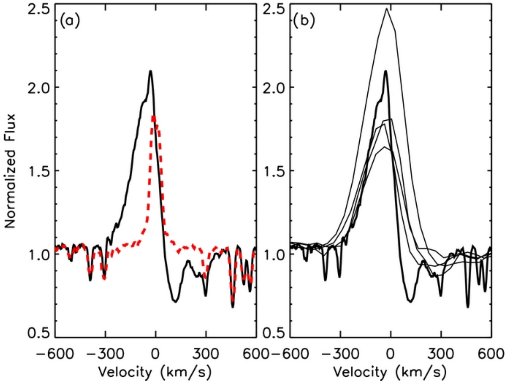
Figure 2. from Near-ultraviolet Excess in Slowly Accreting T Tauri Stars: Limits Imposed by Chromospheric Emission Ingleby et al. 2011 ApJ 743 105 doi:10.1088/0004-637X/743/2/105 https://dx.doi.org/10.1088/0004-637X/743/2/105 © 2011. The American Astronomical Society. All rights reserved.
