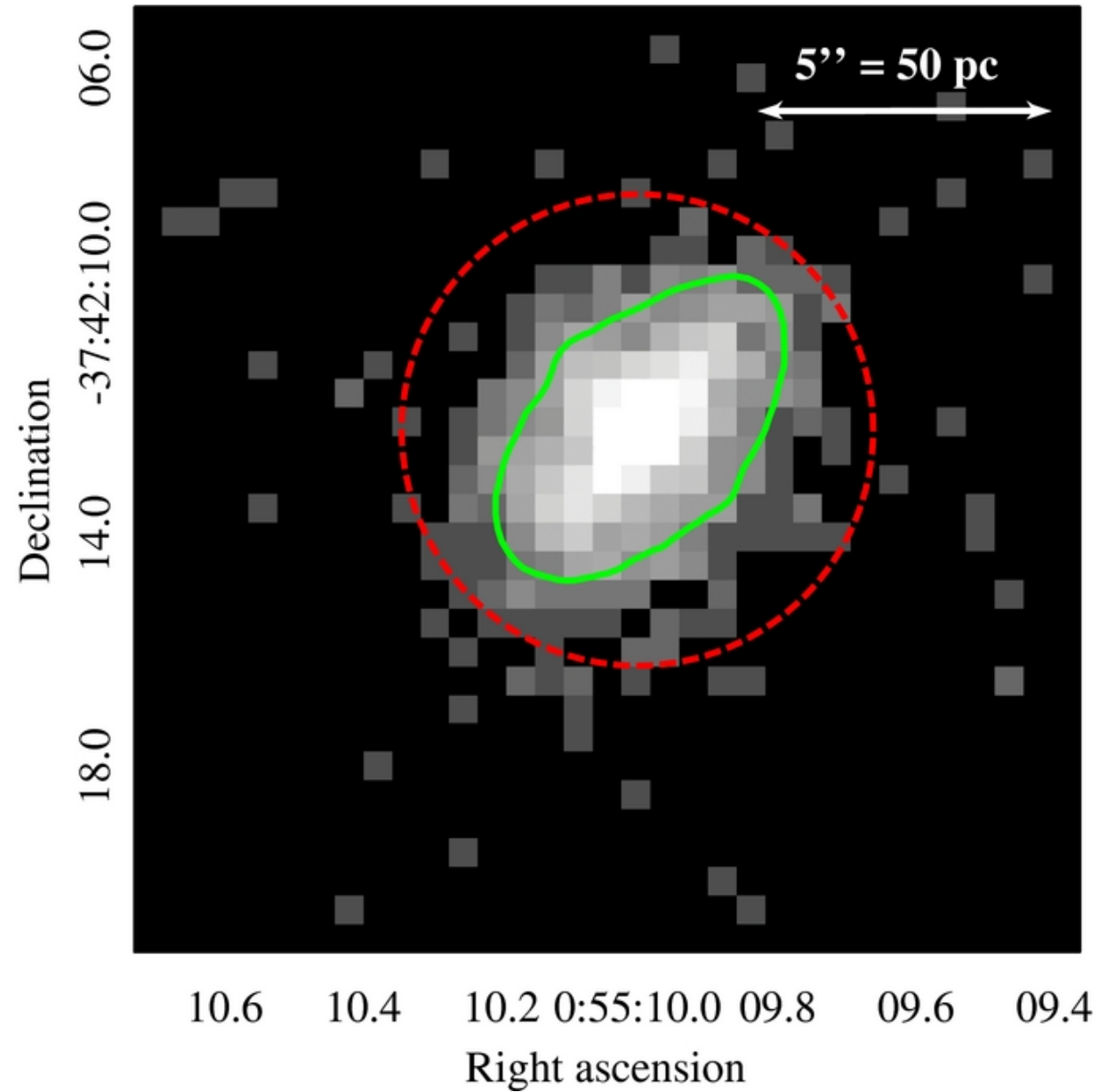
Figure 1. from A Deep Chandra Observation of the Wolf-Rayet + Black Hole Binary NGC 300 X-1 Binder et al. 2011 ApJ 742 128 doi:10.1088/0004-637X/742/2/128 https://dx.doi.org/10.1088/0004-637X/742/2/128 © 2011. The American Astronomical Society. All rights reserved.
