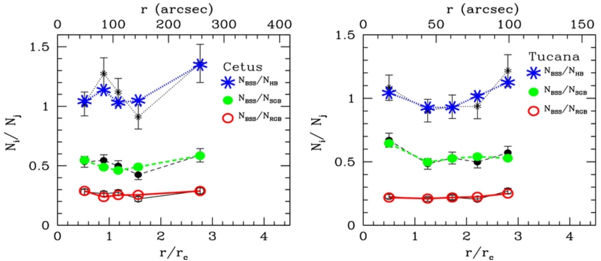
Figure 9. from The ACS LCID Project. VII. The Blue Stragglers Population in the Isolated dSph Galaxies Cetus and Tucana Monelli et al. 2012 ApJ 744 157 doi:10.1088/0004-637X/744/2/157 https://dx.doi.org/10.1088/0004-637X/744/2/157 © 2012. The American Astronomical Society. All rights reserved.
