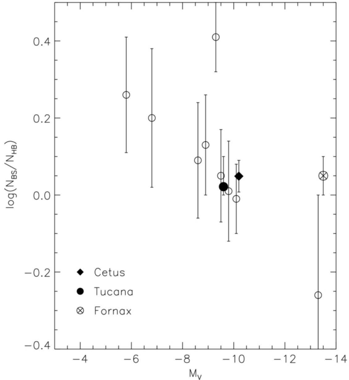
Figure 7. from The ACS LCID Project. VII. The Blue Stragglers Population in the Isolated dSph Galaxies Cetus and Tucana Monelli et al. 2012 ApJ 744 157 doi:10.1088/0004-637X/744/2/157 https://dx.doi.org/10.1088/0004-637X/744/2/157 © 2012. The American Astronomical Society. All rights reserved.
