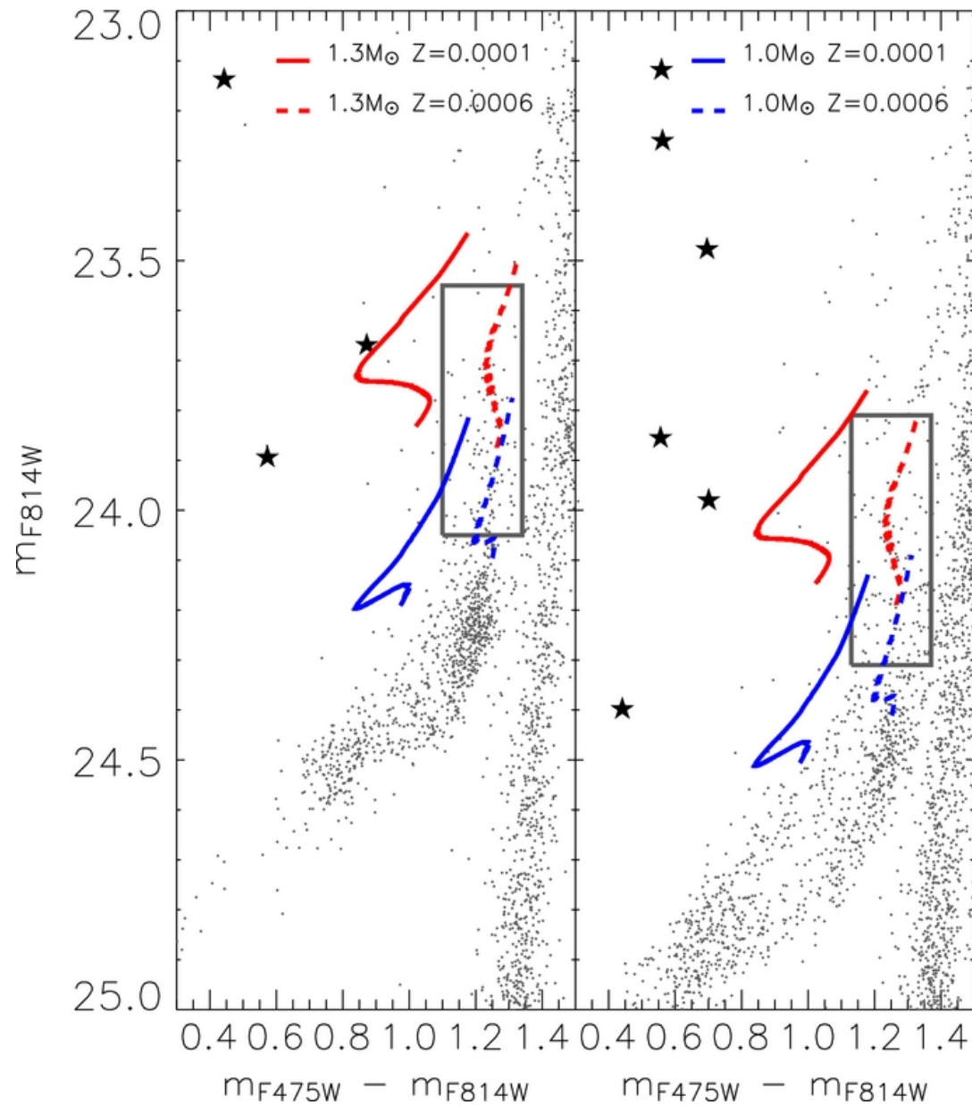
Figure 3. from The ACS LCID Project. VII. The Blue Stragglers Population in the Isolated dSph Galaxies Cetus and Tucana Monelli et al. 2012 ApJ 744 157 doi:10.1088/0004-637X/744/2/157 https://dx.doi.org/10.1088/0004-637X/744/2/157
