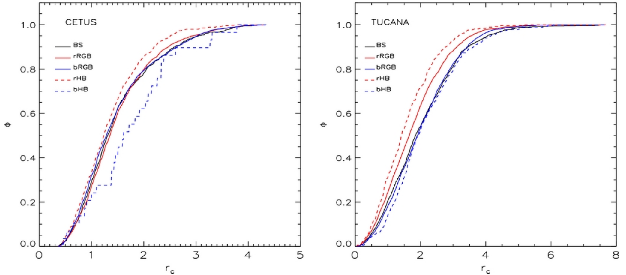
Figure 13. from The ACS LCID Project. VII. The Blue Stragglers Population in the Isolated dSph Galaxies Cetus and Tucana Monelli et al. 2012 ApJ 744 157 doi:10.1088/0004-637X/744/2/157 https://dx.doi.org/10.1088/0004-637X/744/2/157 © 2012. The American Astronomical Society. All rights reserved.
