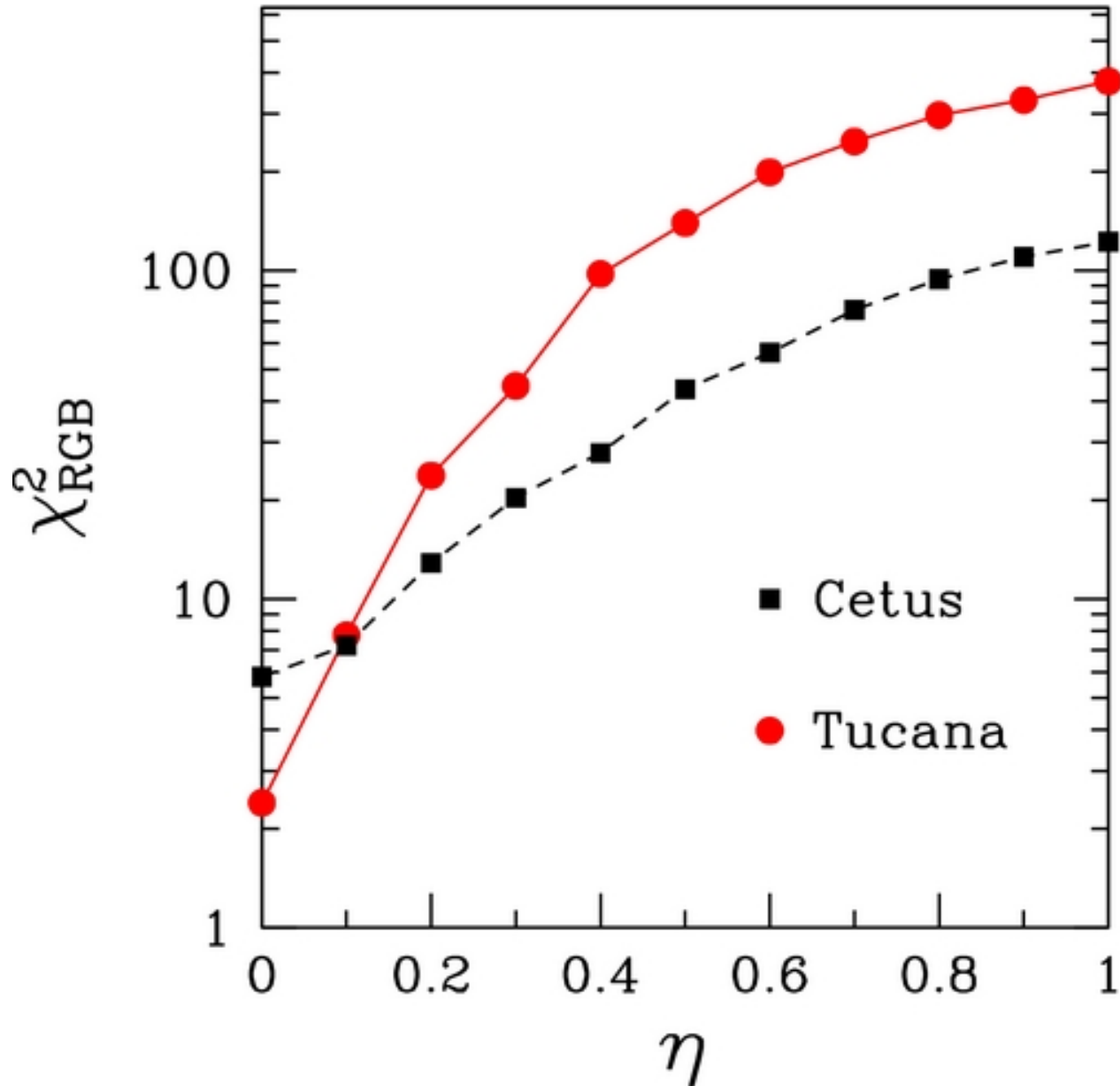
Figure 10. from The ACS LCID Project. VII. The Blue Stragglers Population in the Isolated dSph Galaxies Cetus and Tucana Monelli et al. 2012 ApJ 744 157 doi:10.1088/0004-637X/744/2/157 https://dx.doi.org/10.1088/0004-637X/744/2/157 © 2012. The American Astronomical Society. All rights reserved.
