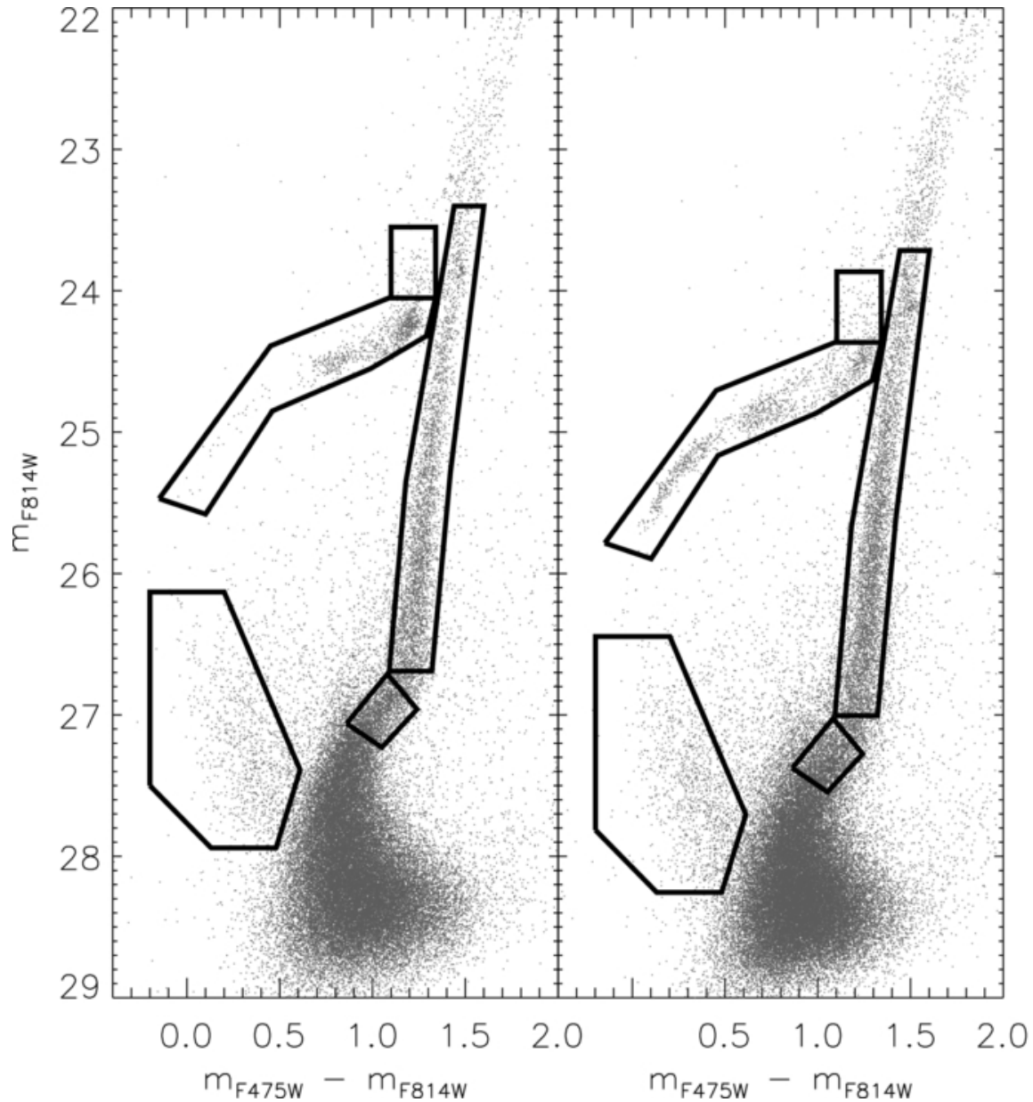
Figure 1. from The ACS LCID Project. VII. The Blue Stragglers Population in the Isolated dSph Galaxies Cetus and Tucana Monelli et al. 2012 ApJ 744 157 doi:10.1088/0004-637X/744/2/157 https://dx.doi.org/10.1088/0004-637X/744/2/157 © 2012. The American Astronomical Society. All rights reserved.
