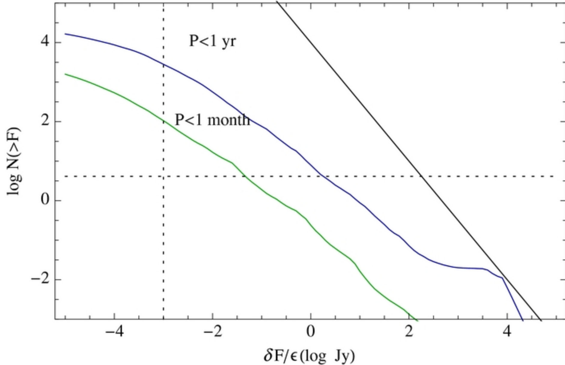
Figure 5. from Blindly Detecting Orbital Modulations of Jets from Merging Supermassive Black Holes O'Shaughnessy et al. 2011 ApJ 743 136 doi:10.1088/0004-637X/743/2/136 https://dx.doi.org/10.1088/0004-637X/743/2/136 © 2011. The American Astronomical Society. All rights reserved.
