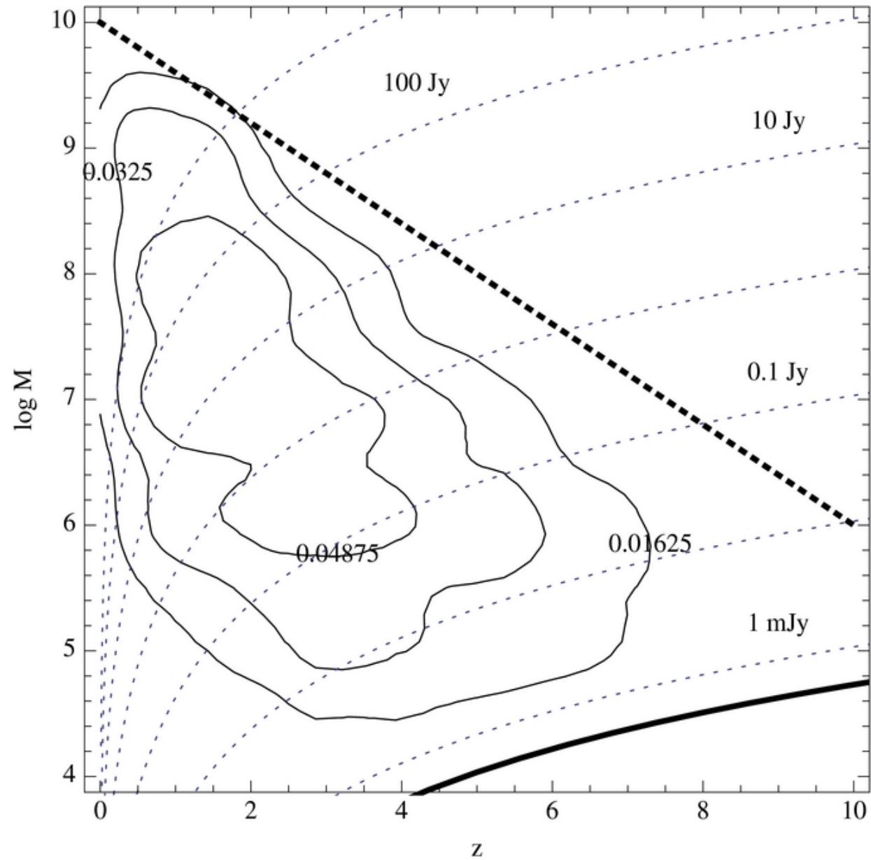
Figure 4. from Blindly Detecting Orbital Modulations of Jets from Merging Supermassive Black Holes O'Shaughnessy et al. 2011 ApJ 743 136 doi:10.1088/0004-637X/743/2/136 https://dx.doi.org/10.1088/0004-637X/743/2/136 © 2011. The American Astronomical Society. All rights reserved.
