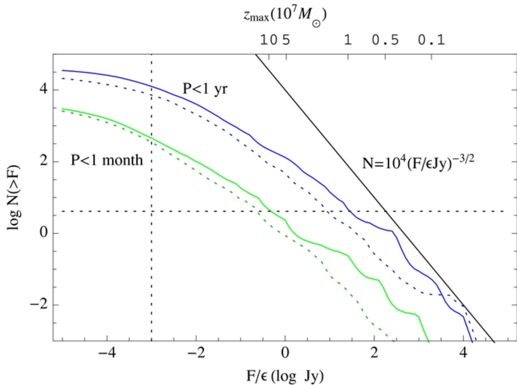
Figure 3. from Blindly Detecting Orbital Modulations of Jets from Merging Supermassive Black Holes O'Shaughnessy et al. 2011 ApJ 743 136 doi:10.1088/0004-637X/743/2/136 https://dx.doi.org/10.1088/0004-637X/743/2/136 © 2011. The American Astronomical Society. All rights reserved.
