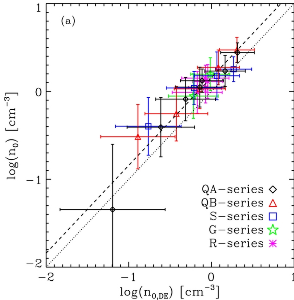
Figure 9. from Regulation of Star Formation Rates in Multiphase Galactic Disks: Numerical Tests of the Thermal/Dynamical Equilibrium Model Kim, Kim, & Ostriker 2011 ApJ 743 25 doi:10.1088/0004-637X/743/1/25 https://dx.doi.org/10.1088/0004-637X/743/1/25 © 2011. The American Astronomical Society. All rights reserved.
