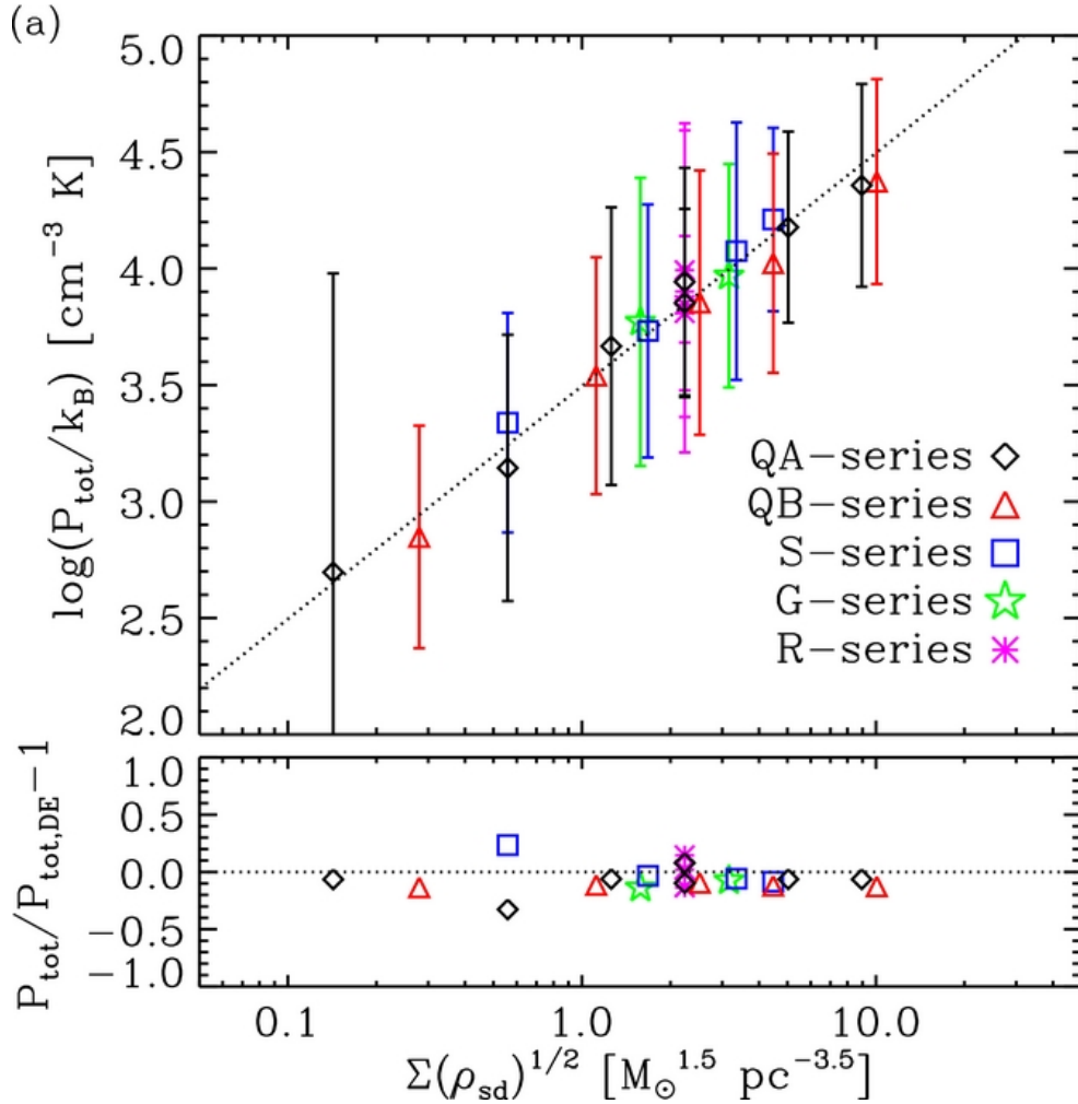
Figure 8. from Regulation of Star Formation Rates in Multiphase Galactic Disks: Numerical Tests of the Thermal/Dynamical Equilibrium Model Kim, Kim, & Ostriker 2011 ApJ 743 25 doi:10.1088/0004-637X/743/1/25 https://dx.doi.org/10.1088/0004-637X/743/1/25 © 2011. The American Astronomical Society. All rights reserved.
