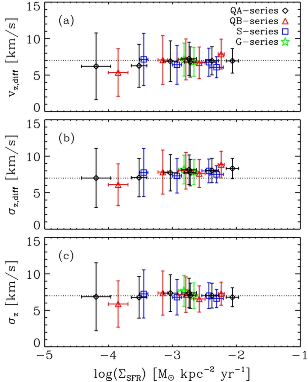
Figure 6. from Regulation of Star Formation Rates in Multiphase Galactic Disks: Numerical Tests of the Thermal/Dynamical Equilibrium Model Kim, Kim, & Ostriker 2011 ApJ 743 25 doi:10.1088/0004-637X/743/1/25 https://dx.doi.org/10.1088/0004-637X/743/1/25
