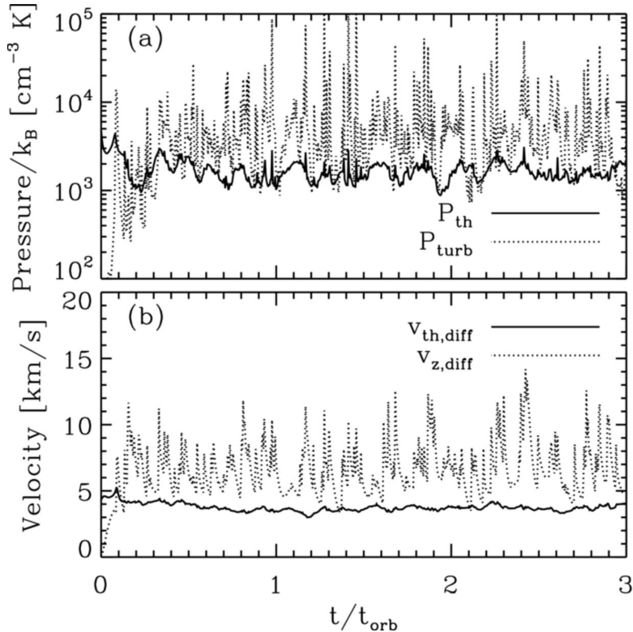
Figure 5. from Regulation of Star Formation Rates in Multiphase Galactic Disks: Numerical Tests of the Thermal/Dynamical Equilibrium Model Kim, Kim, & Ostriker 2011 ApJ 743 25 doi:10.1088/0004-637X/743/1/25 https://dx.doi.org/10.1088/0004-637X/743/1/25 © 2011. The American Astronomical Society. All rights reserved.
