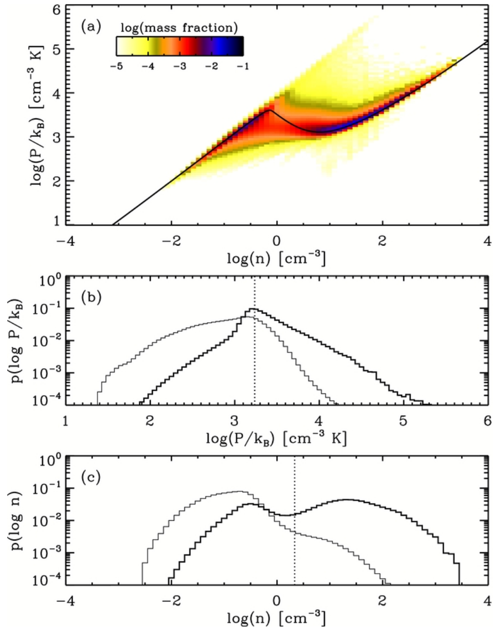
Figure 4. from Regulation of Star Formation Rates in Multiphase Galactic Disks: Numerical Tests of the Thermal/Dynamical Equilibrium Model Kim, Kim, & Ostriker 2011 ApJ 743 25 doi:10.1088/0004-637X/743/1/25 https://dx.doi.org/10.1088/0004-637X/743/1/25
