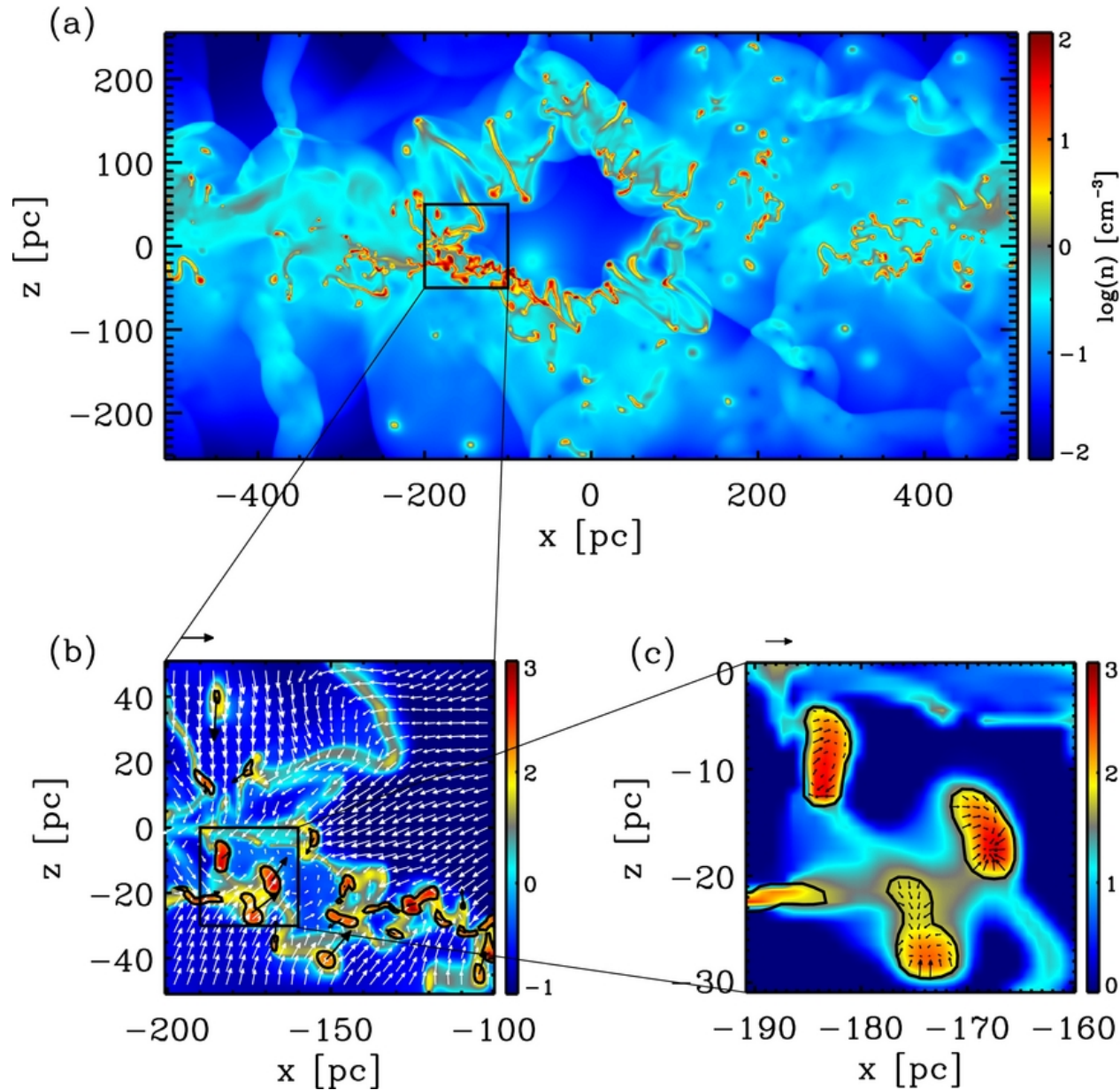
Figure 3. from Regulation of Star Formation Rates in Multiphase Galactic Disks: Numerical Tests of the Thermal/Dynamical Equilibrium Model Kim, Kim, & Ostriker 2011 ApJ 743 25 doi:10.1088/0004-637X/743/1/25 https://dx.doi.org/10.1088/0004-637X/743/1/25 © 2011. The American Astronomical Society. All rights reserved.
