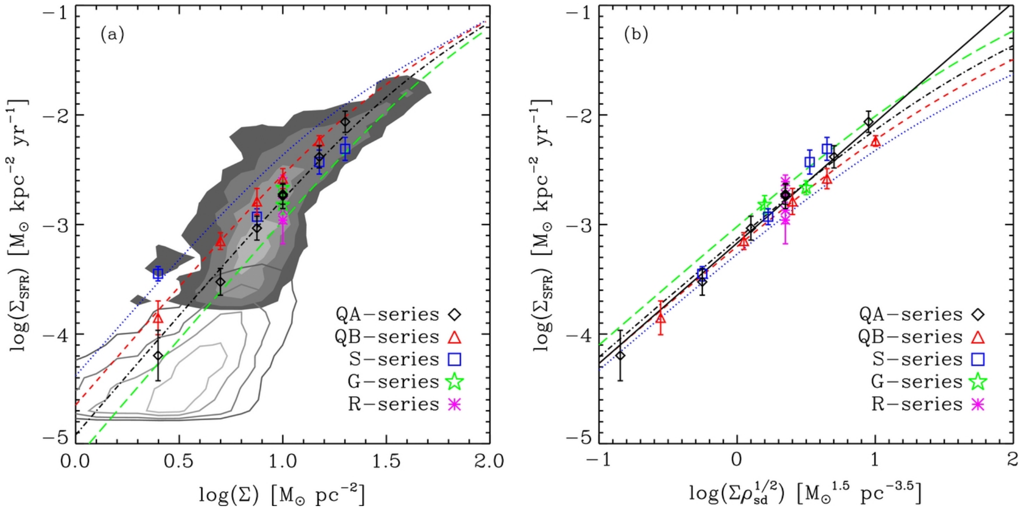
Figure 13. from Regulation of Star Formation Rates in Multiphase Galactic Disks: Numerical Tests of the Thermal/Dynamical Equilibrium Model Kim, Kim, & Ostriker 2011 ApJ 743 25 doi:10.1088/0004-637X/743/1/25 https://dx.doi.org/10.1088/0004-637X/743/1/25 © 2011. The American Astronomical Society. All rights reserved.
