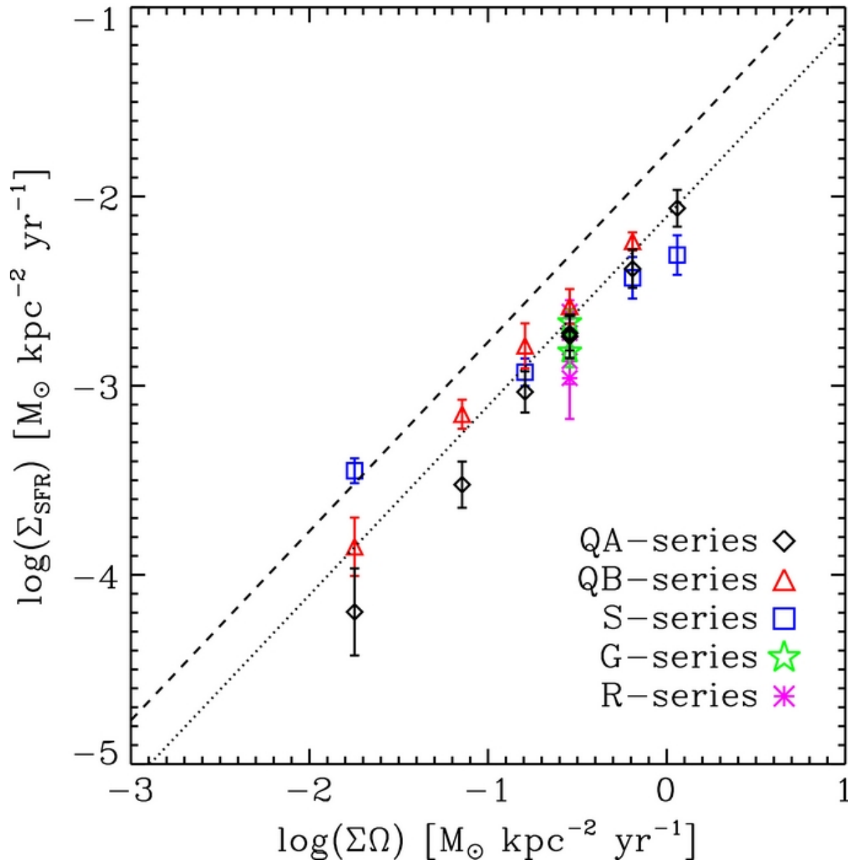
Figure 12. from Regulation of Star Formation Rates in Multiphase Galactic Disks: Numerical Tests of the Thermal/Dynamical Equilibrium Model Kim, Kim, & Ostriker 2011 ApJ 743 25 doi:10.1088/0004-637X/743/1/25 https://dx.doi.org/10.1088/0004-637X/743/1/25 © 2011. The American Astronomical Society. All rights reserved.
